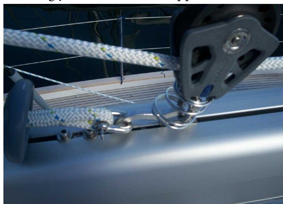
Correct position – shackle will not scratch the boom
