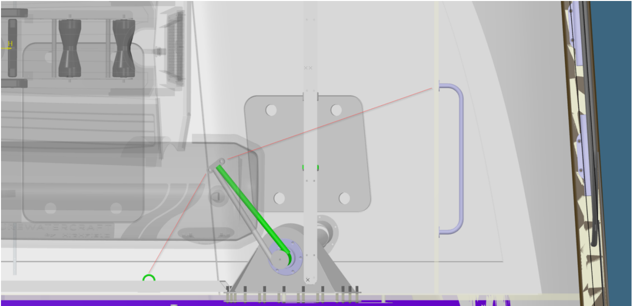
Hallberg-Rassy 69, emergency steering arrangement in aft lazarette
