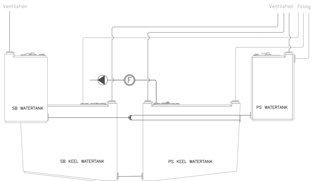
Principle drawing Fresh water system HR 69
